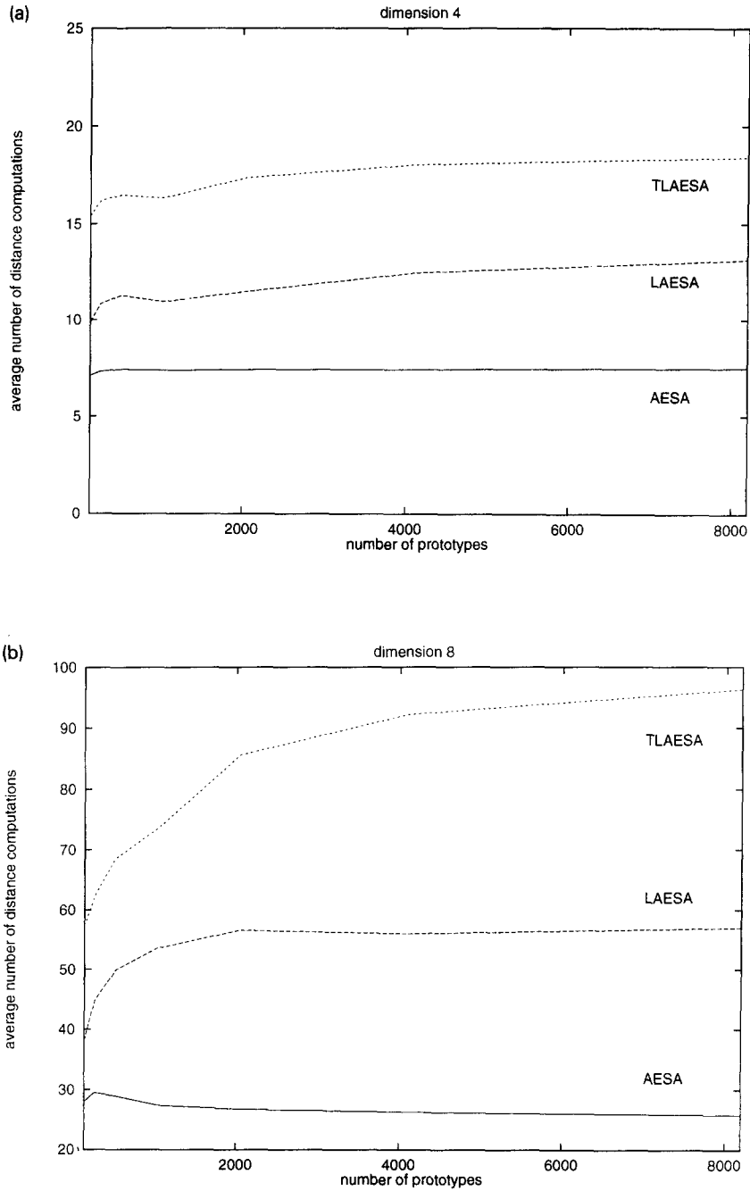
Fig. 7. Comparison of the results with TLAES in Fig. 5 with the corresponding results using AESA and LAESA.
